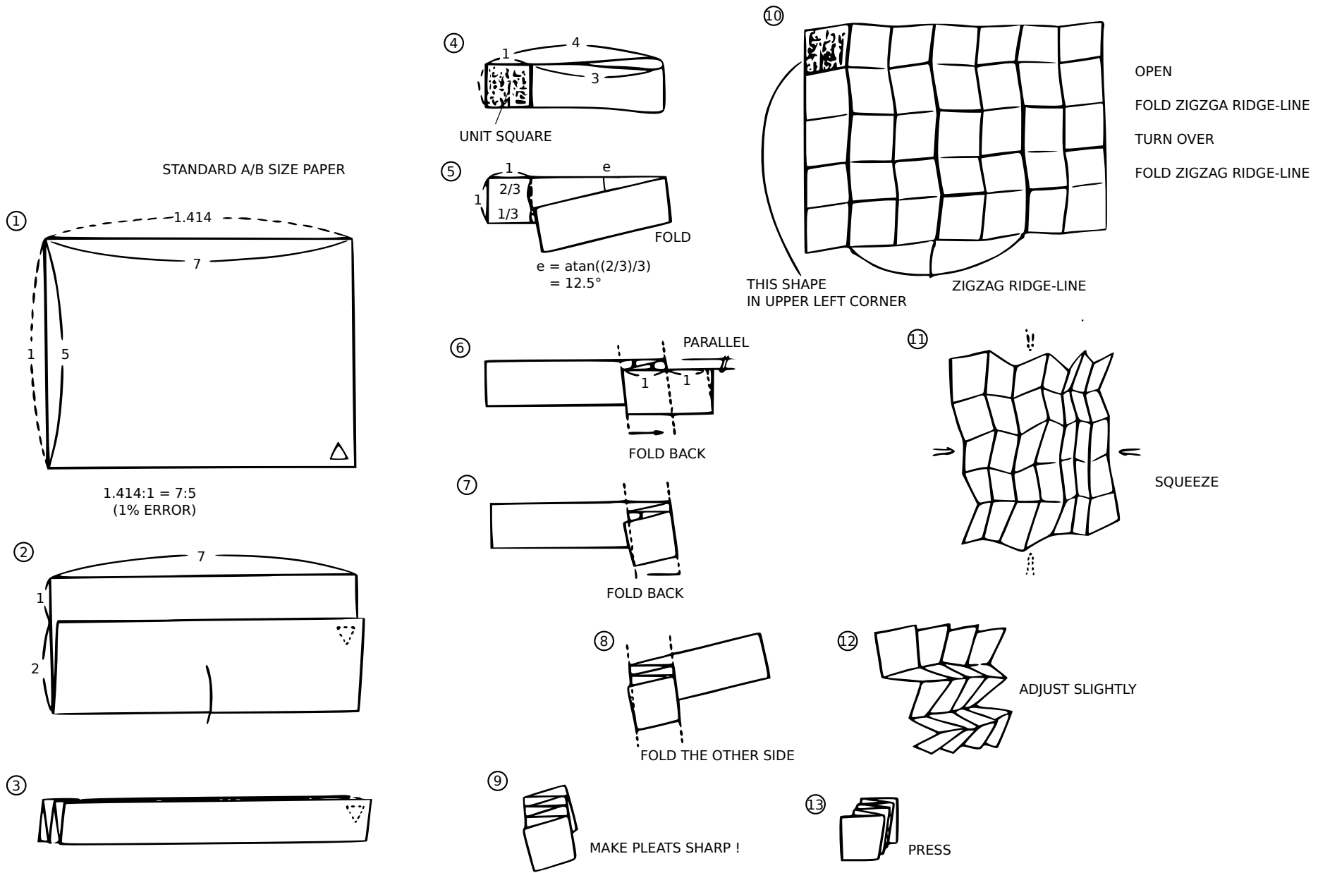
Fig. 10. How to fold Miura-ori, Natori's method (Illustration by M. Sakamaki).
